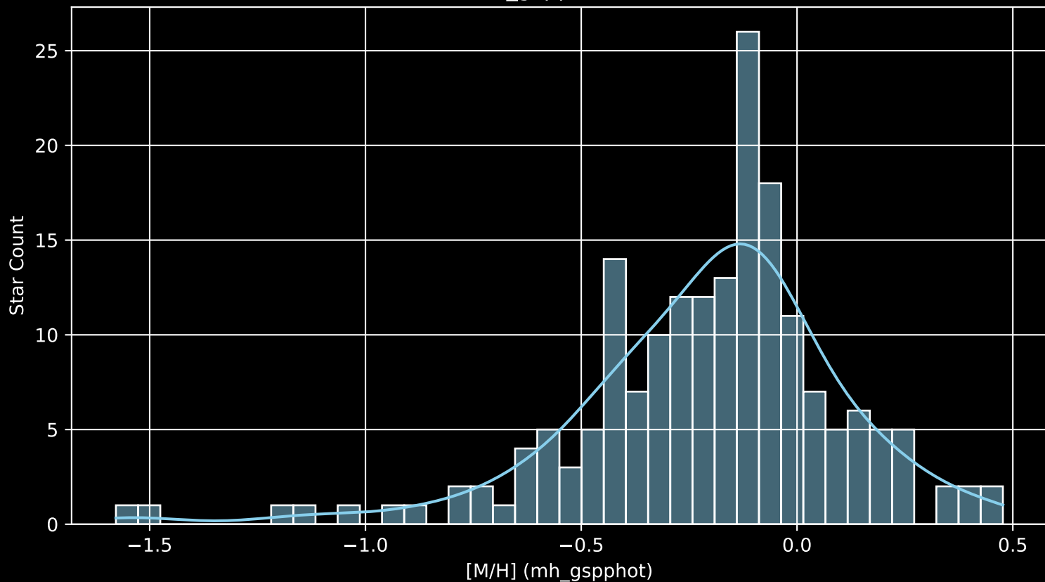
APOGEE DR17 Field: [CVZ_OB19_btx [M/H] (mh_gspphot) (n= 186)
