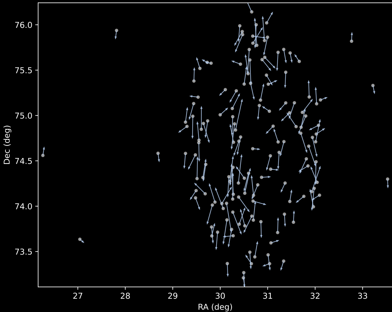
APOGEE DR17 Cluster 1 Proper Motion Vectors (n=146)
