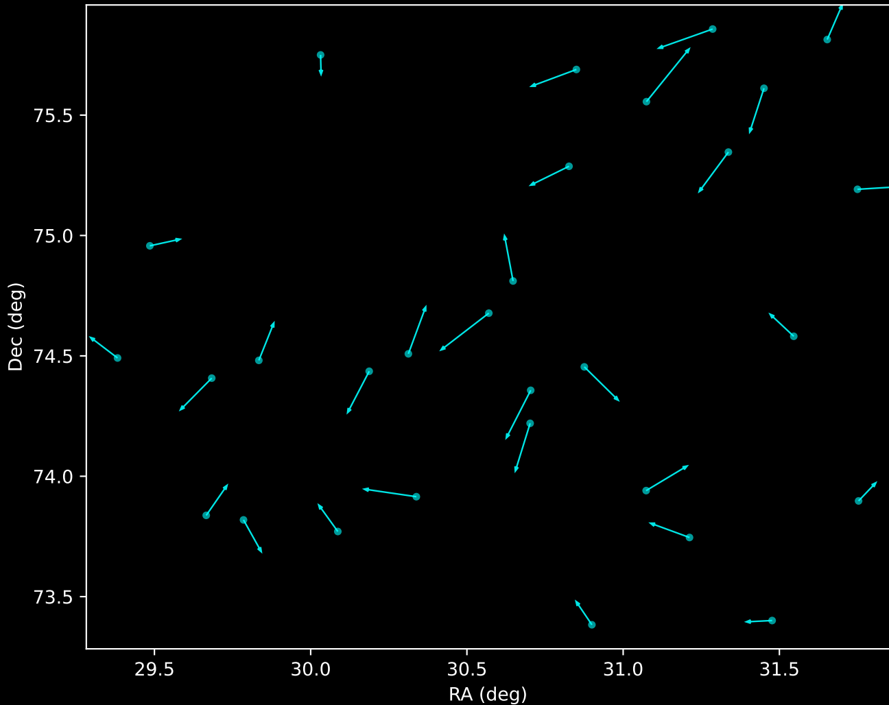
APOGEE DR17 Noise Stream Proper Motion Vectors (n=30)
