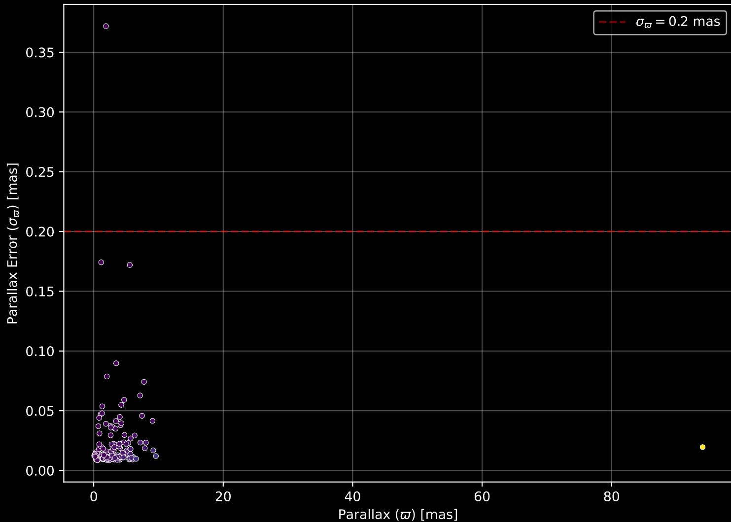
APOGEE DR17 Field: [CVZ_OB19_btx] Parallax Quality (n= 187)
