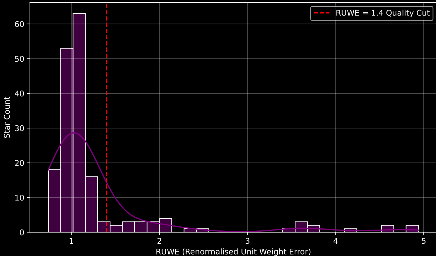
GAPOGEE DR17 Field [CVZ_OB19_btx] RUWE Distribution (n= 181)
