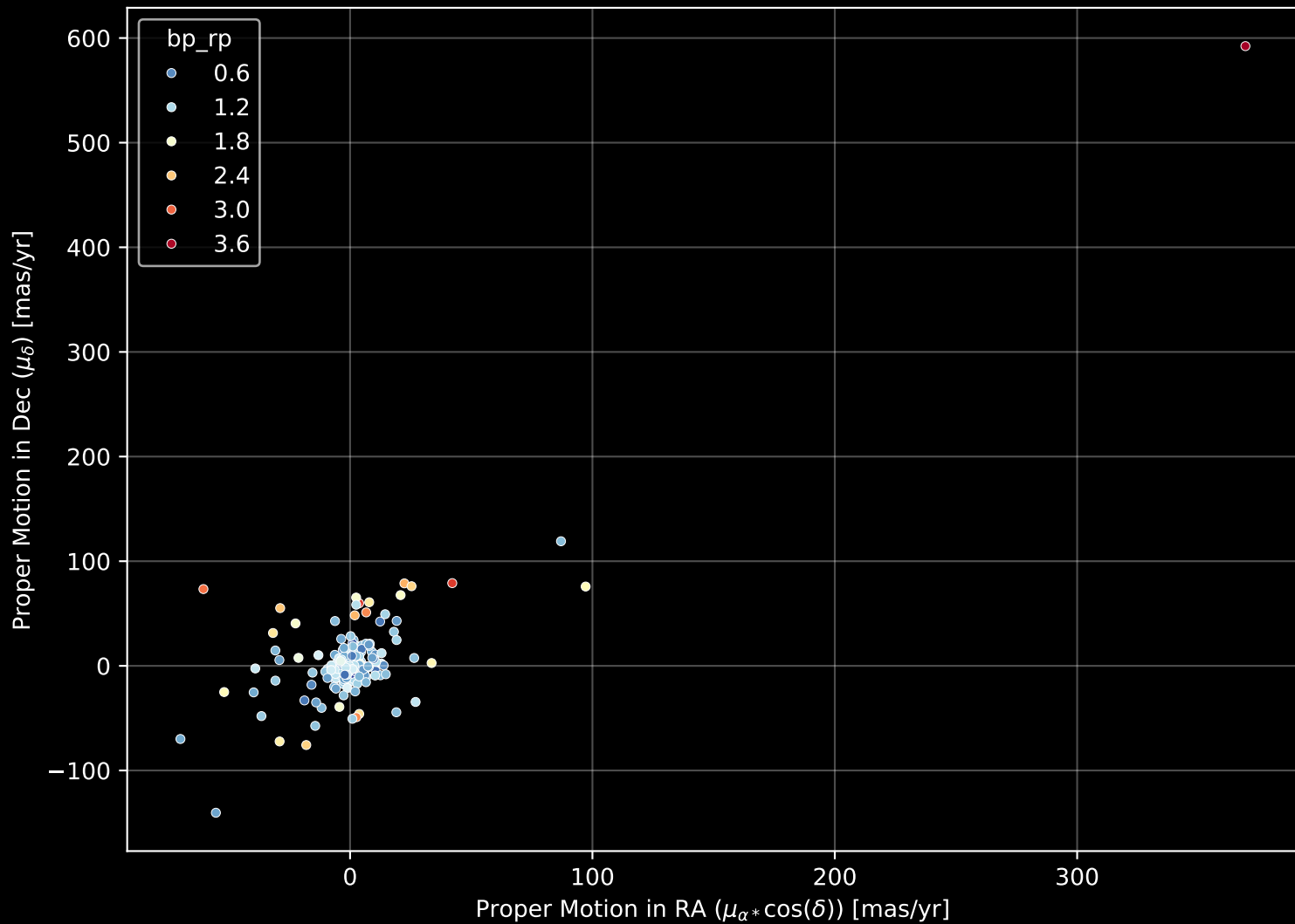
APOGEE DR17 Field: [CVZ_OB19_btx] Proper Motion Diagram (n= 187)
