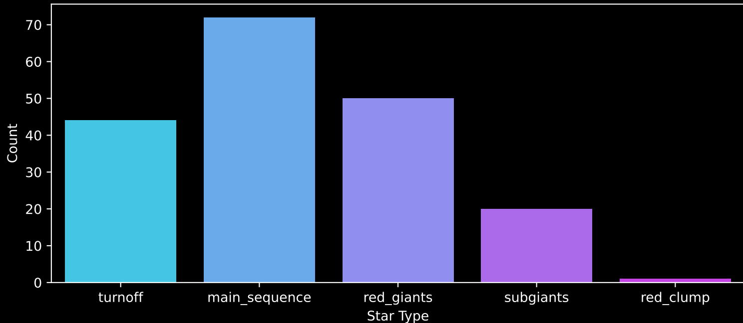
APOGEE DR17 Field: [CVZ_OB19_btx] Count plot of Star Type
