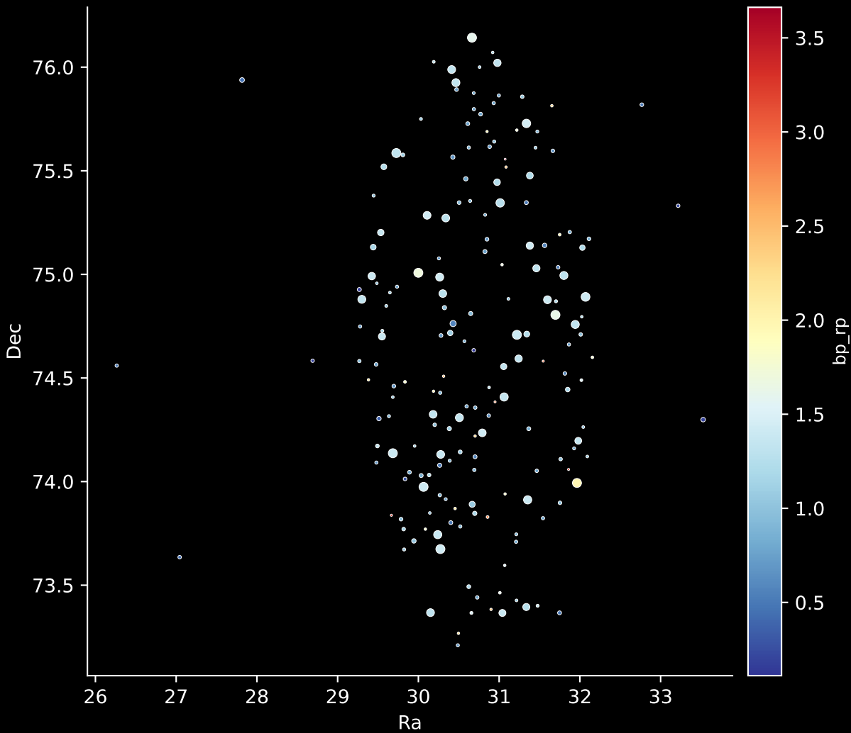
APOGEE DR17 Field: [CVZ_OB19_btx] Stars: 187
